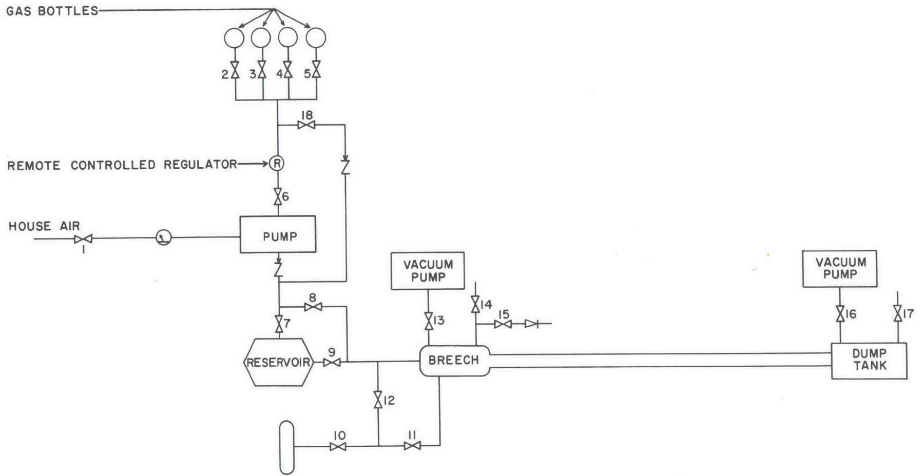
Fig. 13. Gas flow circuit.
